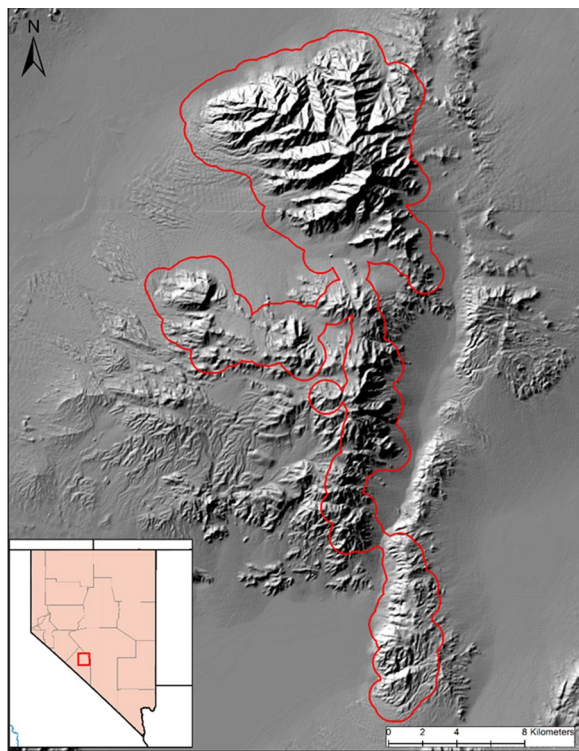
Fig. 2 Map of the Lone Mountain study area in west central Nevada. The red boundary in the main figure represents the area defined as available for bighorn sheep (2016–2018). The red square in the inset figure shows the study area location within Nevada in addition to the state counties
