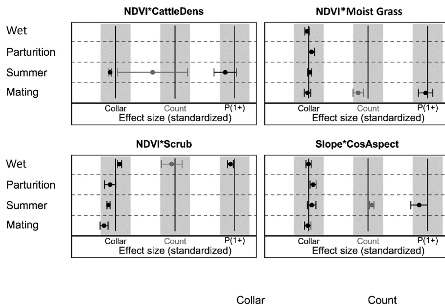
Fig. B1. Interactions between covariates related to patterns of habitat selection by tule elk. Vertical lines indicate an effect size of zero, and gray regions represent (standardized) effect sizes between -2 and 2 . Collar : modeled from GPS collar data collected at Point Reyes National Seashore from November 2012 to March 2018 (see Appendix A for details). Count and P(1+) : Modeled from visual surveys conducted at Point Reyes National Seashore from September 2010 to November 2017. Count represents probability that elk abundance will increase as a function of each covariate. P(1+) represents probability of elk presence (one or more elk observed) as a function of each covariate. Error bars represent 1 standard error (s.e.).
